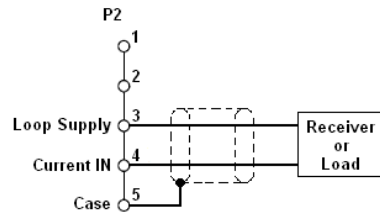
4.20mA OUTPUT USING THE INTERNAL LOOP SUPPLY
