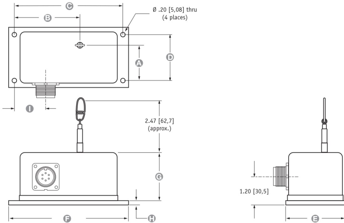
Fig. 1 - Outline Drawing:
