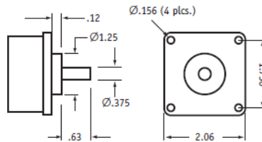
F02 - 2-inch Sq. Flange Mount (3/8-inch shaft)
